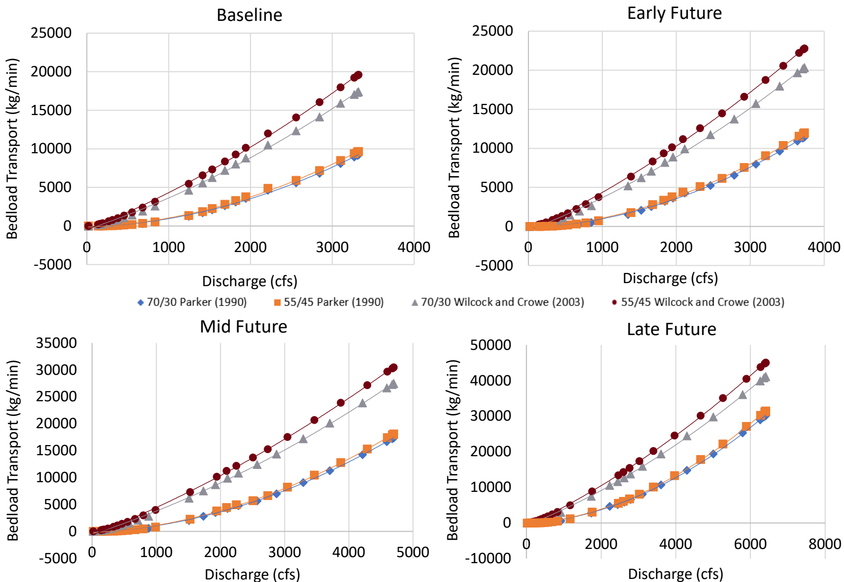
Figure C-15. Cross-Section 52535 Change in Bedload Sediment Transport for a 2-year Return Interval
